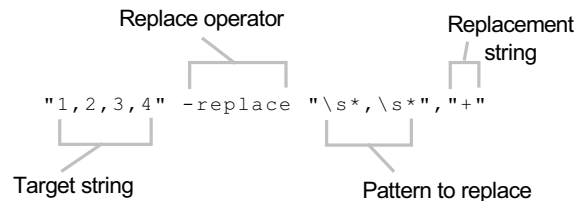
Figure 4.9 The syntax of the -replace operator
