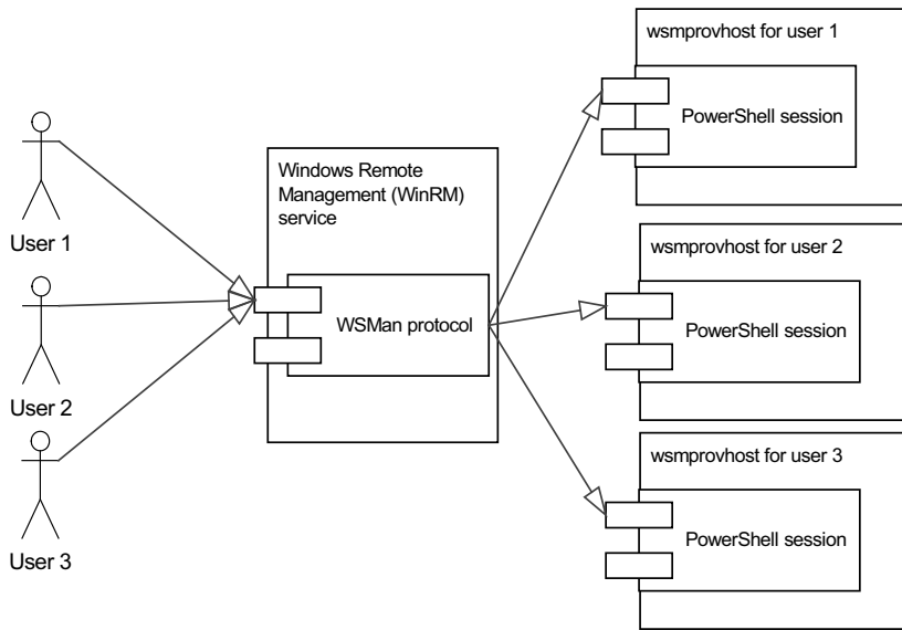
Figure 13.6 When multiple users connect to the WinRM service, a new wsmprovhost process is created to host the PowerShell session for that user. Even when the same user connects multiple times, a new process is still created for each connection.
