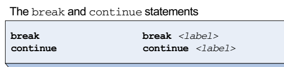
Figure 6.9 The PowerShell break and continue statements, which may optionally take a label indicating which loop statement to break to
